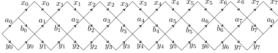
FIGURE 9. The non-positively curved, squared surface \Sigma .
