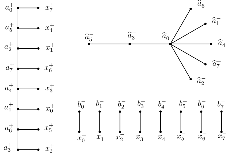
FIGURE 14. Ascending and descending links of v_2 in X .
