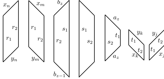
FIGURE 12. The Morse function \widehat{f} on the new 2-cells of C(X) .
