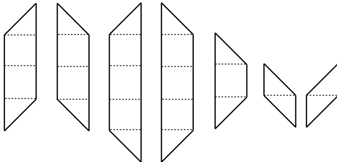
FIGURE 17. Circle vertex preimages in the 2-cells of \Gamma \times [0, 1] (cf. Figure 12).
