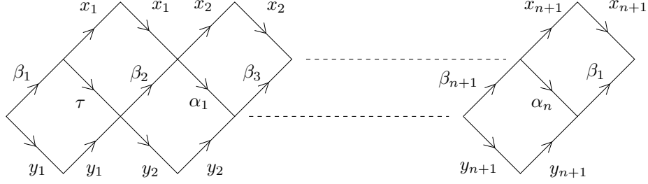
FIGURE 4. The non-positively curved, squared surface \Sigma_n .
