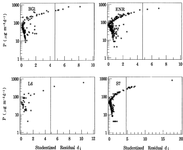
Fig. 4. Examples of outlier detection for the selected sites, where outliers are the right-hand-side data points (*) along the vertical reference (cutoff) line which represents the t -value for \alpha = 0.01 .
