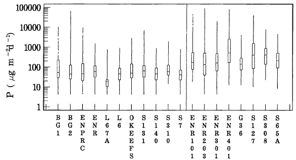
Fig. 3. Box and whisker plots of dry deposition P values from 19 sites in South Florida. The solid line represents the mean at each site, while the middle, bottom and top edges of each box are the median, 25th and 75th percentiles, and the bottom and top of whiskers are the low and high extremes, respectively.
