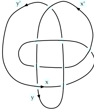
Figure 2: The knot 8_{20}
