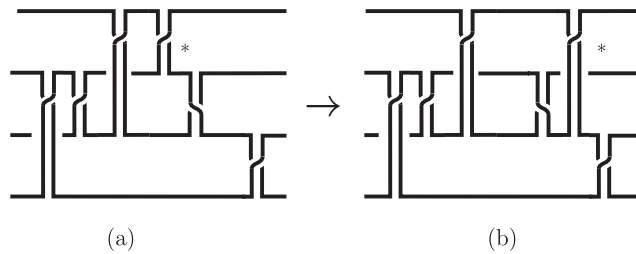
Fig. 5. Deplumbing a Hopf band
