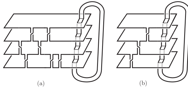
Fig. 2. Seifert surfaces for 3-component links
