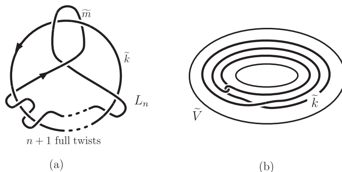
Fig. 8. (a) The link L_n , (b) Pattern when n = 1 .
