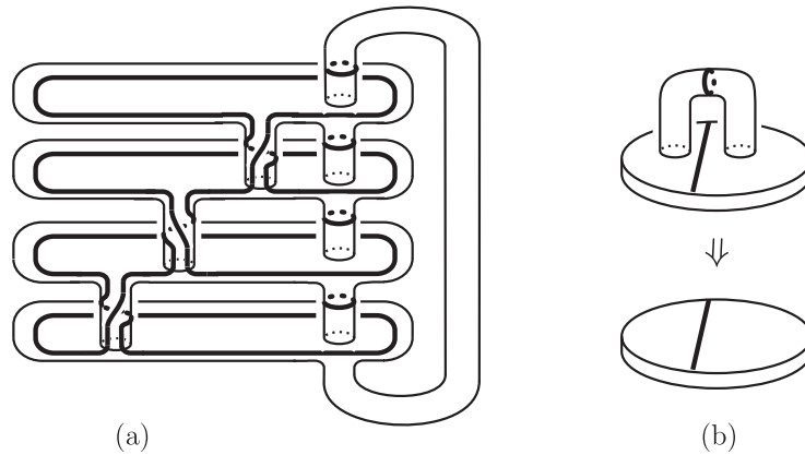
Fig. 3. A sutured manifold and the C -product decomposition
