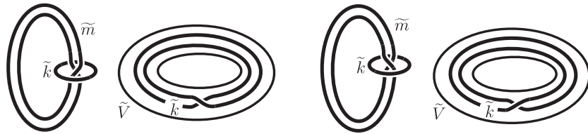
Fig. 7. Fibered patterns of unknot with winding number 2.
