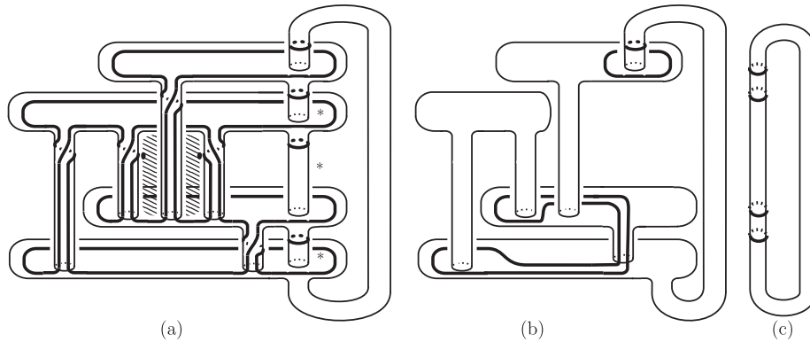
Fig. 6. C-product decompositions
