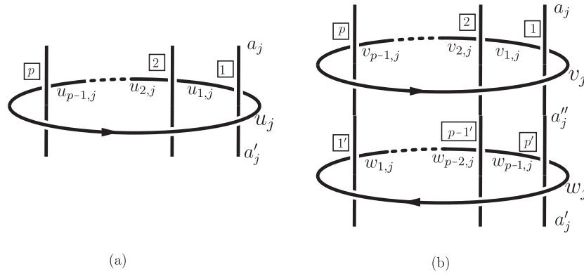
Fig. 1. (a) Partial diagram of \mathcal{D}_1 , (b) Partial diagram of \mathcal{D}_2 .
