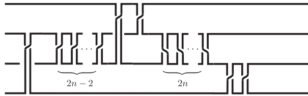
Fig. 4. Seifert surfaces for closed braids
