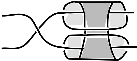
Figure 7: Ribbon disk bounded by staple
