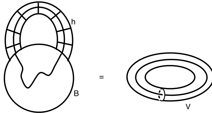
Figure 6: B \cup h seen as solid torus
