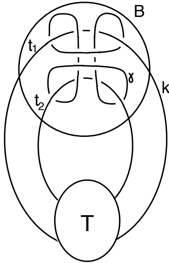
Figure 10: 2-component link L = k \cup \gamma
