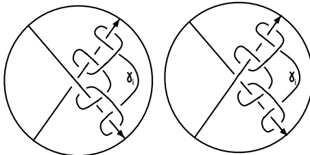
Figure 2: Tangle (B_i, t_i, \gamma_i)
