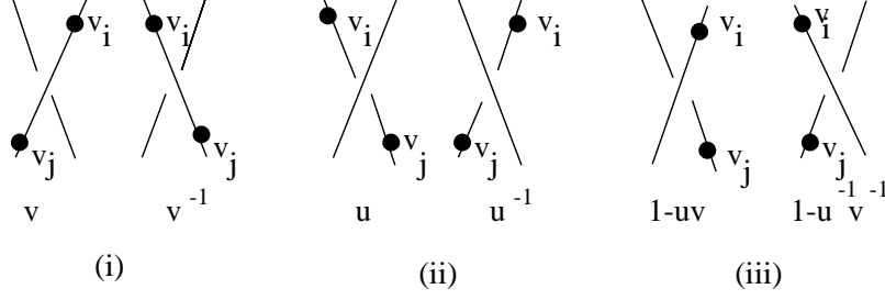
Figure 7: Transitions V_i \rightarrow V_j and Weights
