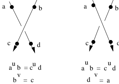
Figure 4: \Lambda -Relations for K
