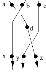
Figure 6: Labeled 3-braid \sigma_1^{-1}\sigma_2
