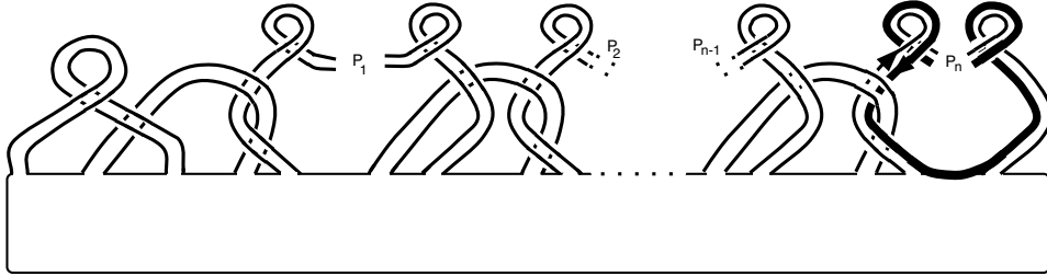
Figure 1: Fibered link from Kanenobu's construction
