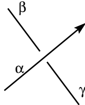
Figure 1: \mathbf{T}^{\mathbf{Z}^d} -Coloring rule
