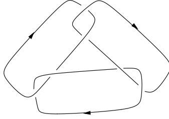
Figure 5: The link l = 6_1^3 .
