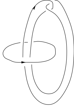
Figure 1: Whitehead link l = 5_1^2
