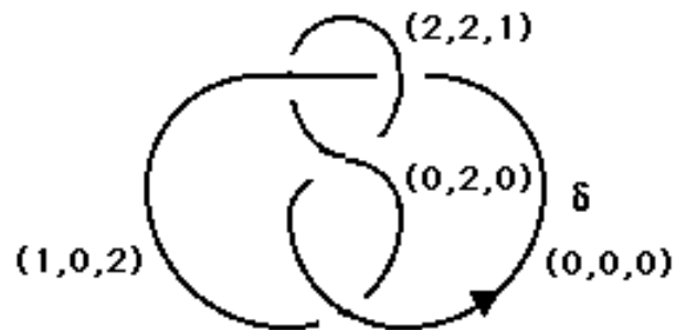
Based (3,4)-coloring of figure eight knot diagram
