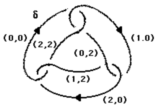
Based (3,3) -coloring of 6_1^3 diagram determined by a nonfixed point
