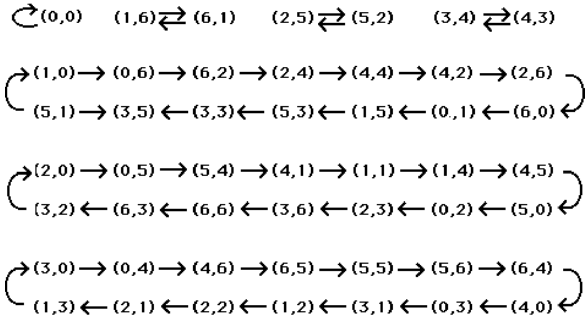
Graph \Gamma for k = 5_2
