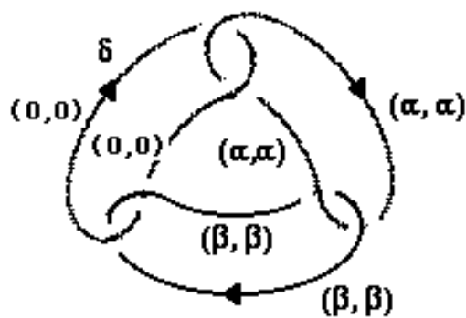
Based (3,3) -coloring of 6_1^3 diagram determined by a fixed point
