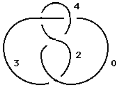
Based 5-coloring of figure eight knot diagram
