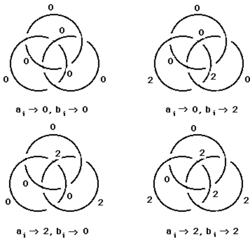
Based (4,2)-colorings of 6_2^3
