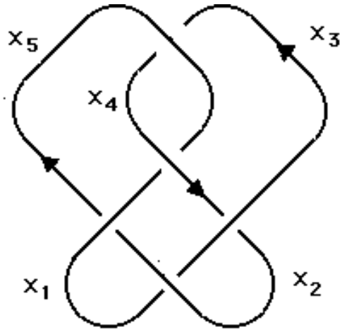
The knot k = 5_2
