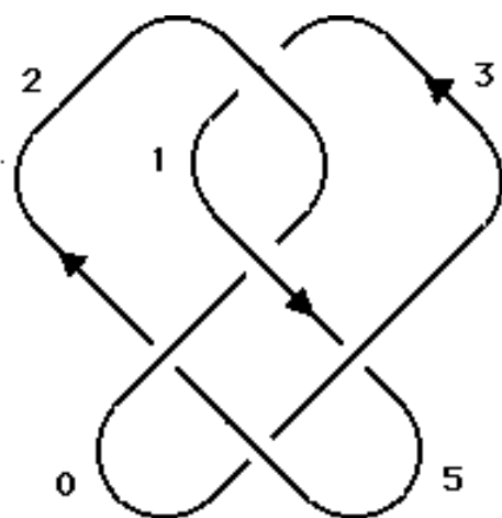
Based (7,2)-coloring of 5_2
