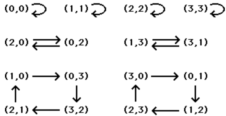
Graph of \Psi
