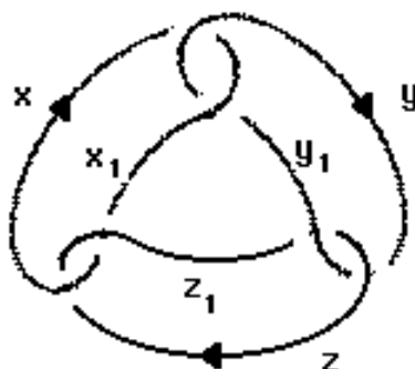
The link 1 = 6_1^3
