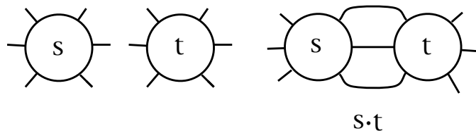
Figure 10: 2n -tangle product
