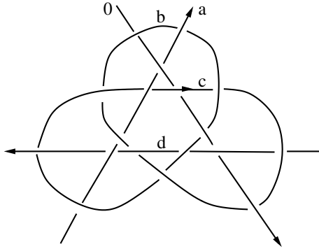
Figure 4: Labeled 6-tangle t
