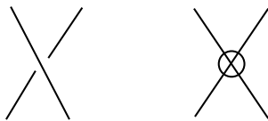
Figure 5: Classical and virtual crossings
