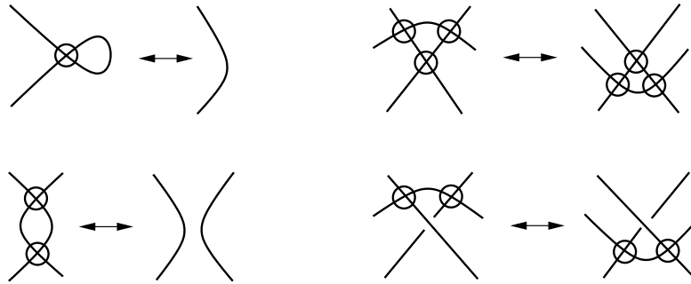
Figure 6: Virtual Reidemeister moves
