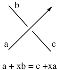
Figure 2. Crossing relation in \mathcal{A}_t
