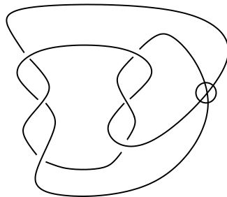
Figure 7: Embedded square-tangle
