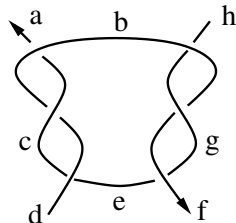
Figure 3: Labeled tangle t
