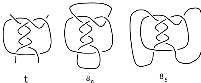
Figure 9: Krebs's tangle and closures
