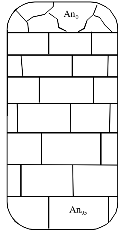
Fractional crystallization of composition M
