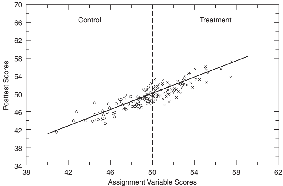
■ FIGURE 10.8 Regression discontinuity experiment with no treatment effects
