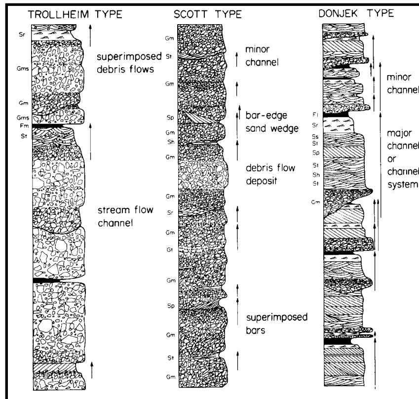
Source: Lewis, D.W., 1984. Practical Sedimentology. Van Nostrand Reinhold, 229p.
