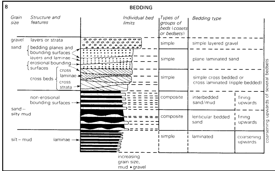
Source: Collinson, J.D. and Thompson, D.B. 1982. Sedimentary Structures. George Allen and Unwin 194p.
