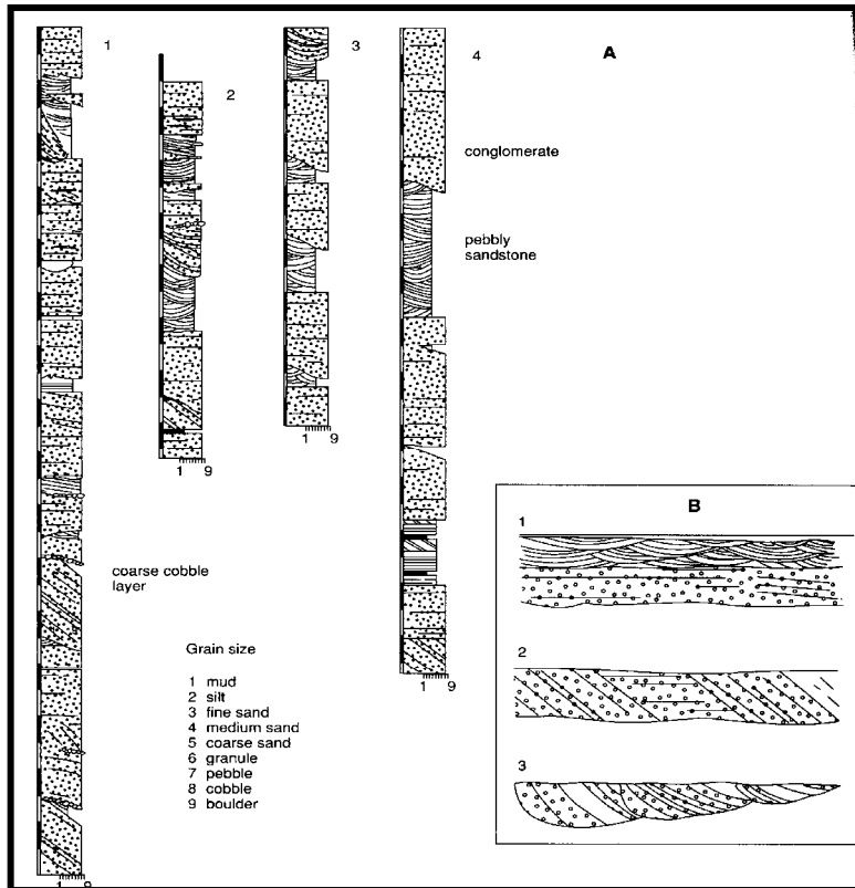
Boggs, S., 1992. Petrology of Sedimentary Rocks. McMillian Publishing, 707 p.
