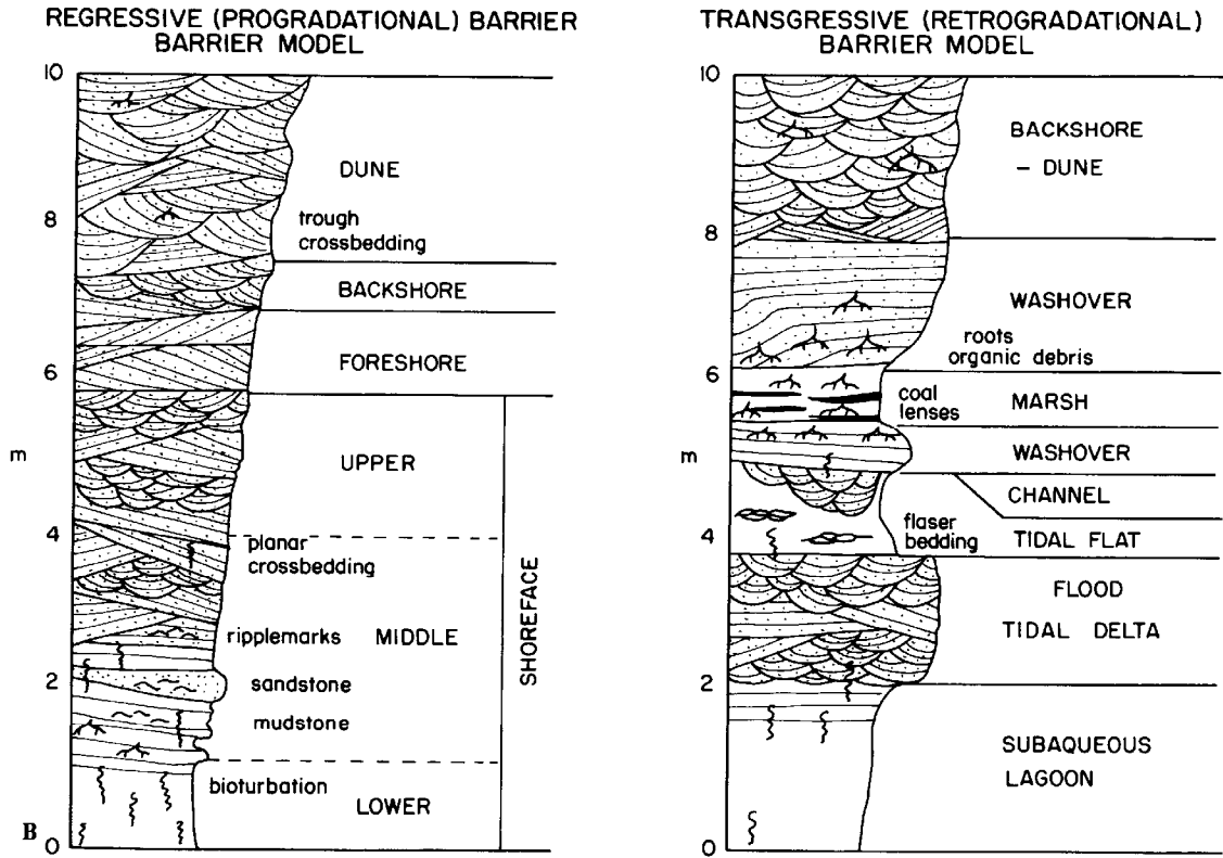
Source: Lewis, D.W., 1984. Practical Sedimentology. Van Nostrand Reinhold, 229p.
