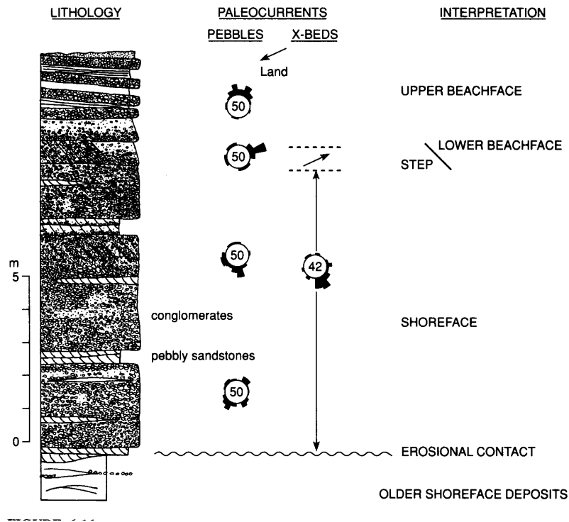
Source: Boggs, S., 1992. Petrology of Sedimentary Rocks. McMillian Publishing, 707 p.
